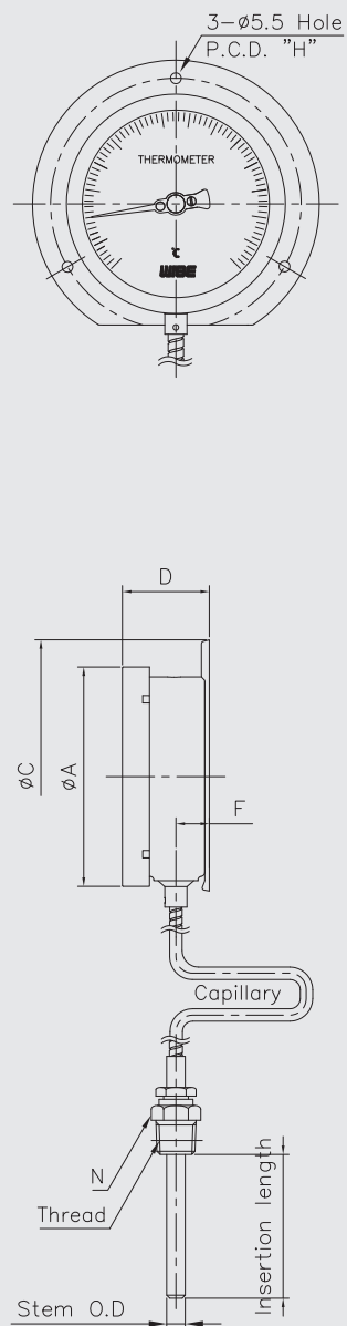
Dimensions (mm)
