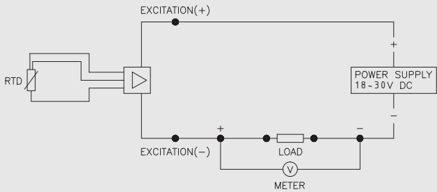
System connection for 2 - wire transmitter
