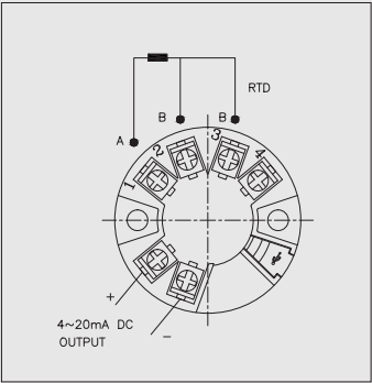
Electrical connection
